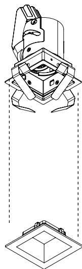
Flanged Trim
