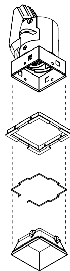
Trimless Millwork
