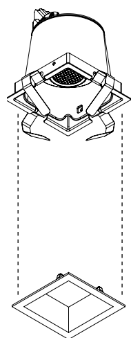
Flanged Trim
