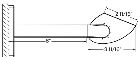
AXLWAI - Axle wall 6" cantilever arm
