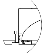
TG15 - tegular 15/16"
