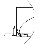
TG9 - tegular 9/16"
