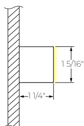
DRYWALL MOUNTING
