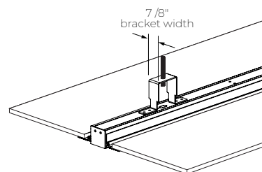
BRACKET SHOW WITH DMF
