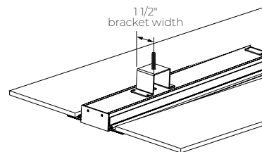
BRACKET SHOWN WITH DMF
