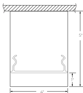
Regressed Lens
