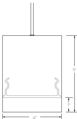
Regressed Lens
