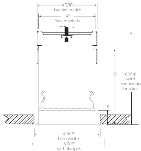
Regressed Lens
