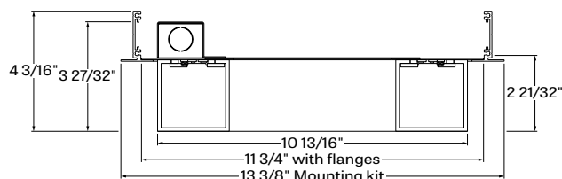
POLRD - recessed drop lens
