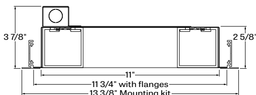
POLRR - recessed regressed lens
