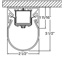
QUANRS - Quad narrow round surface
