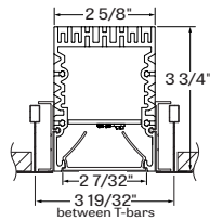
TB15 - T-bar 15/16"
