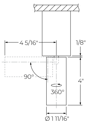
Dot 1.5" - Standard baffle
