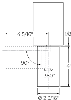
Dot 2" - Standard baffle
