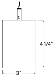
Flush Lens
