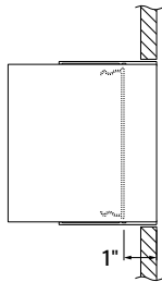
Regressed Lens
