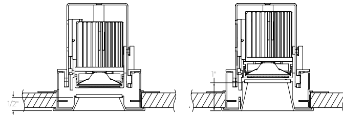
Standard Baffle
